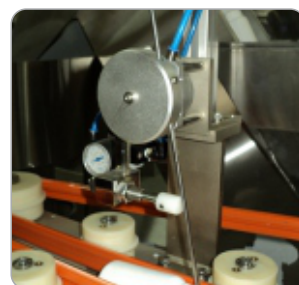
Hook Unit
